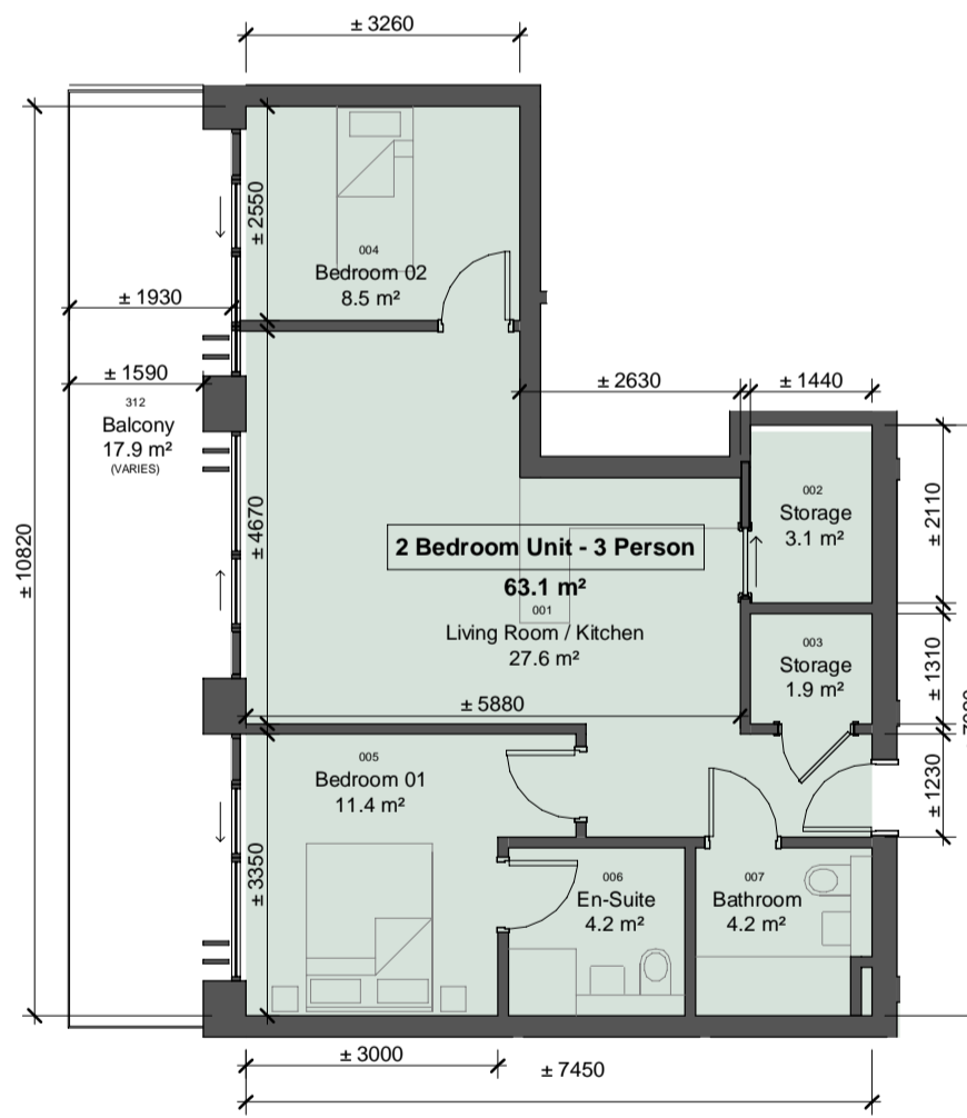
5 Unit Type 2BR-G-1 scale 1 : 100
