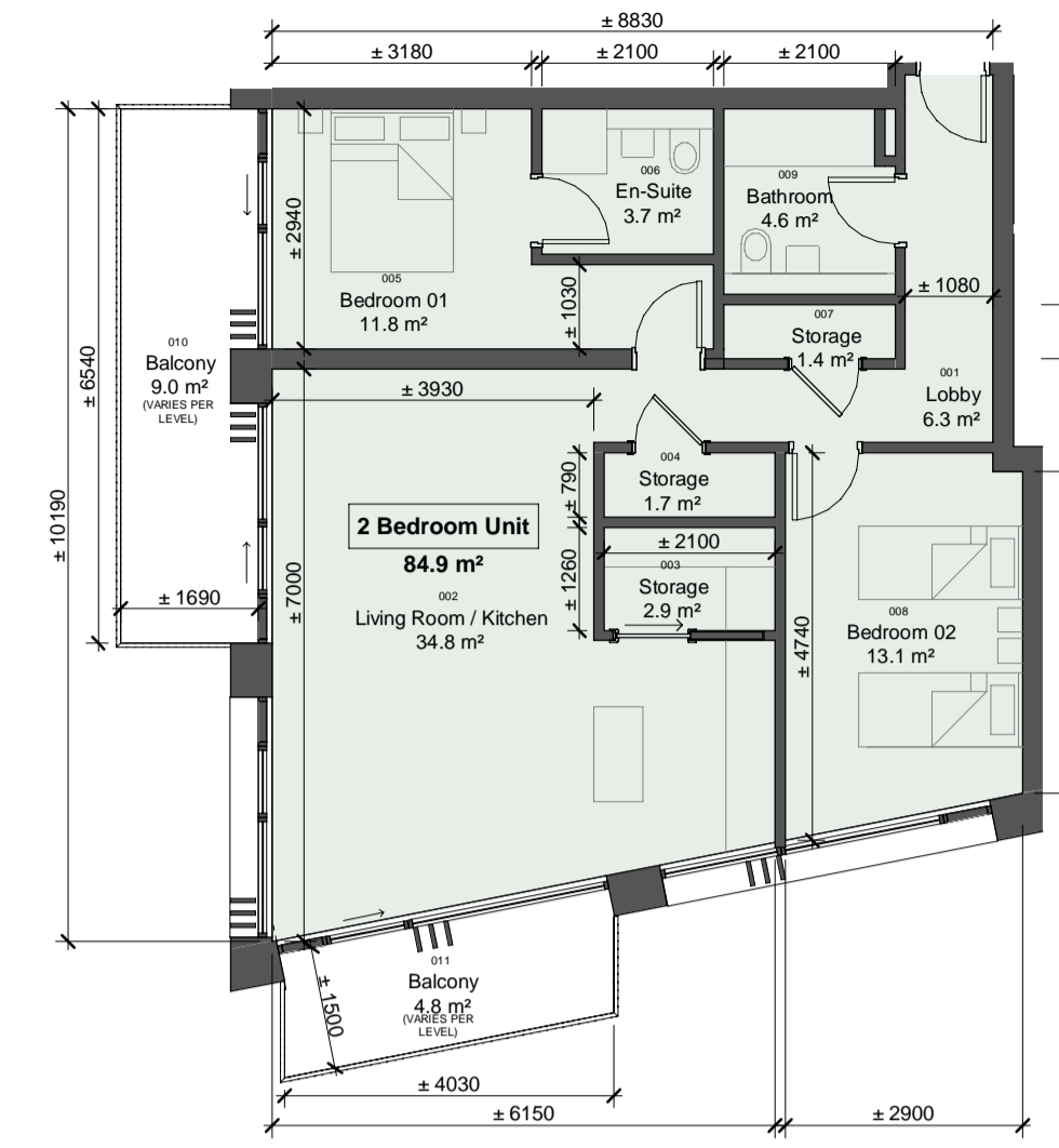
3 Unit Type 2BR-F-1 scale 1 : 100
