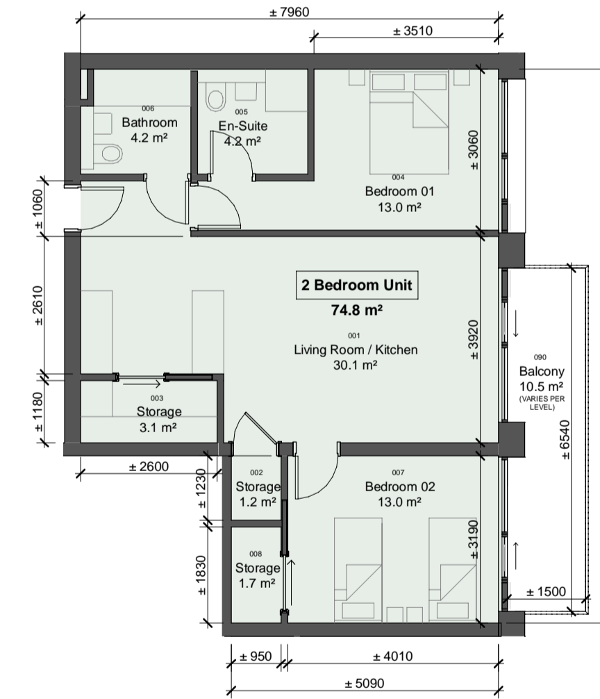
6 Unit Type 2BR-H-1 scale 1 : 100
