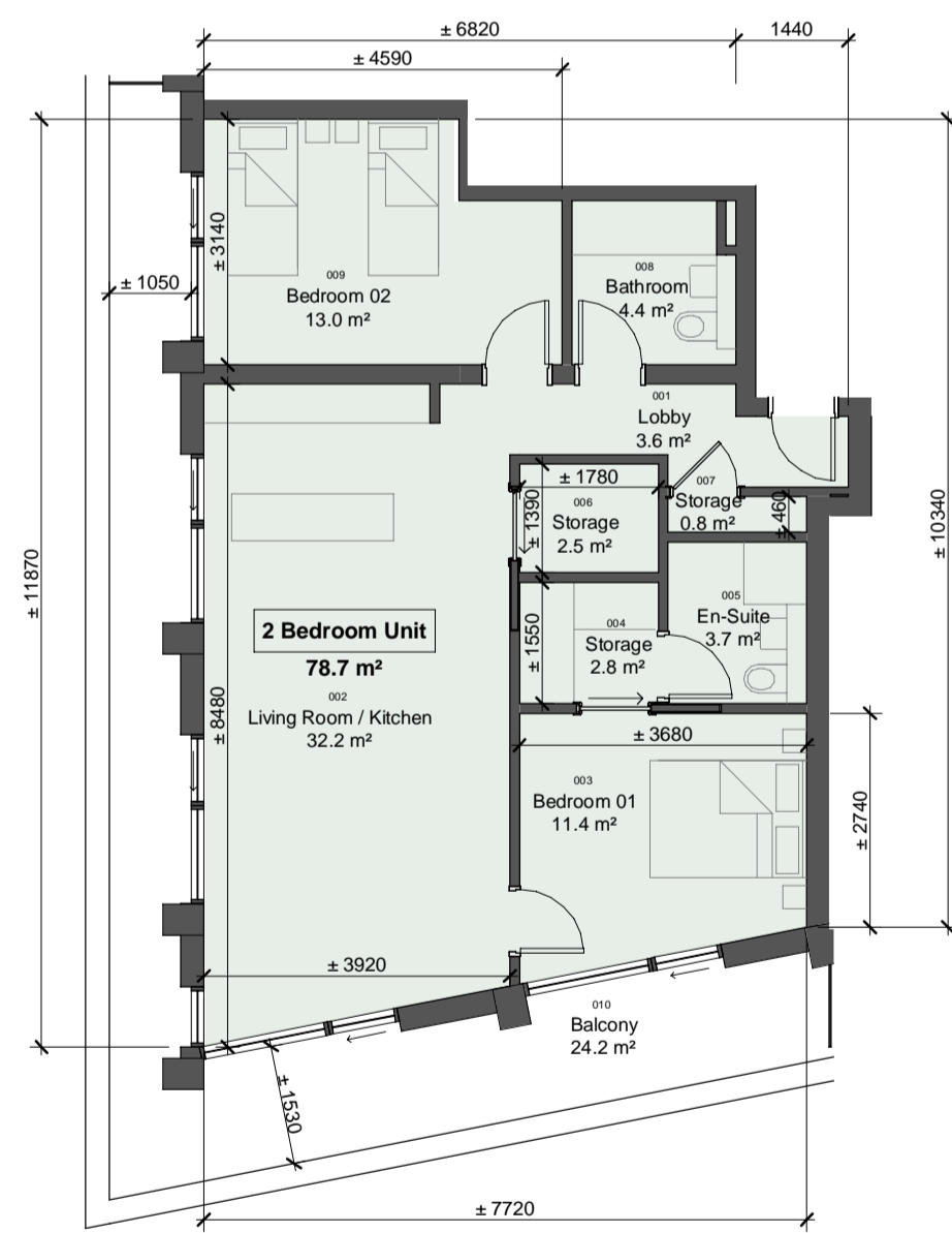
4 Unit Type 2BR-F-2 scale 1 : 100
