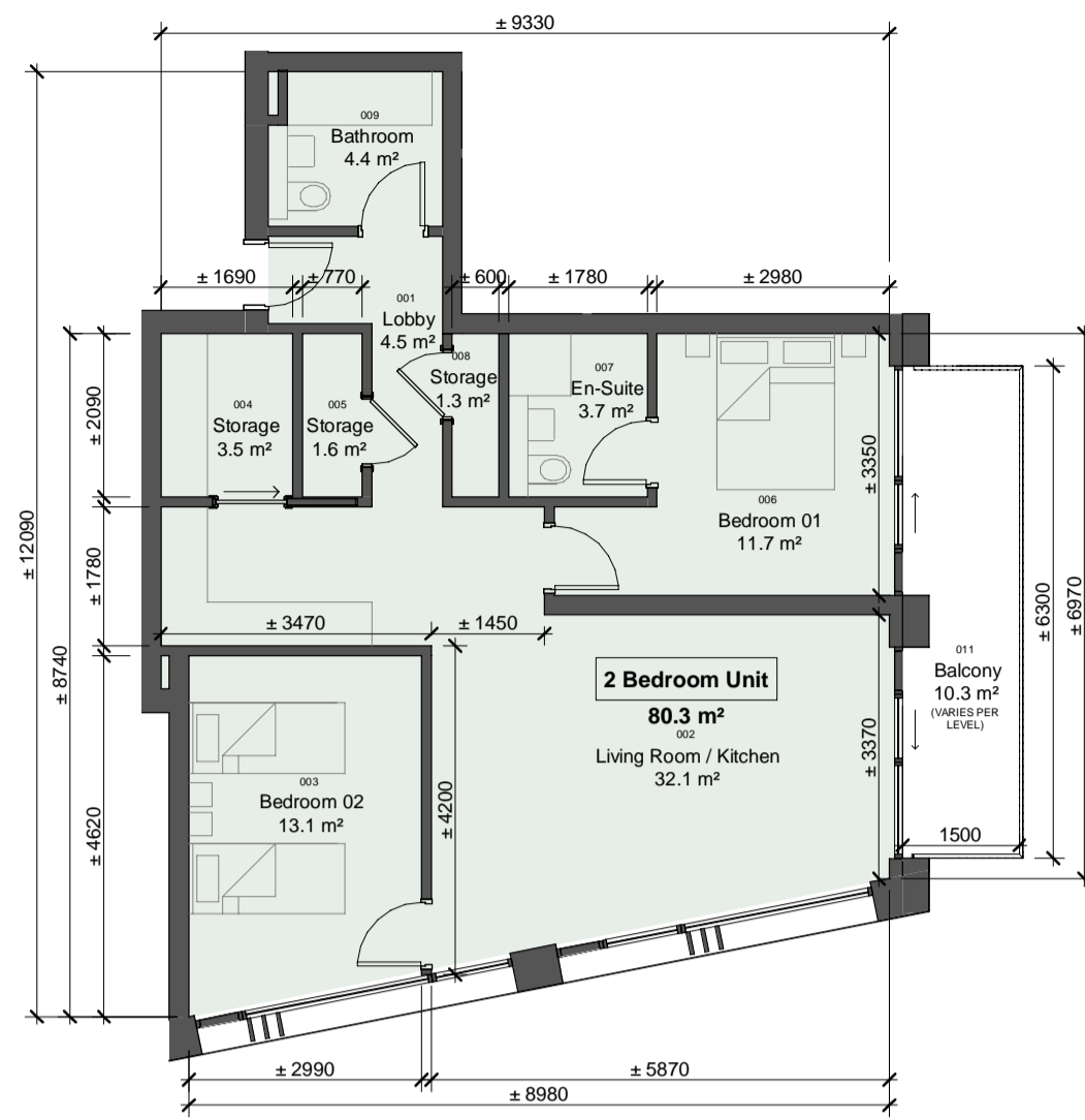
1 Unit Type 2BR-E-1 scale 1 : 100
