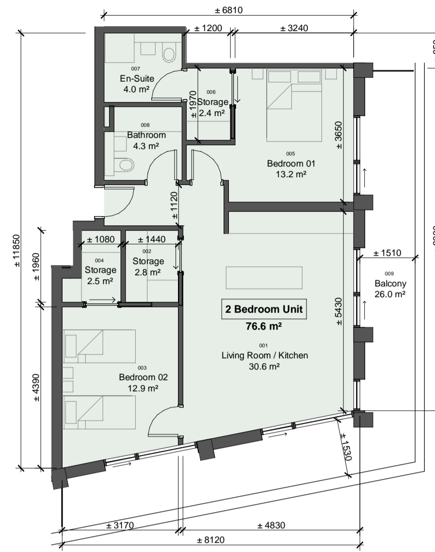
2 Unit Type 2BR-E-2 scale 1 : 100
