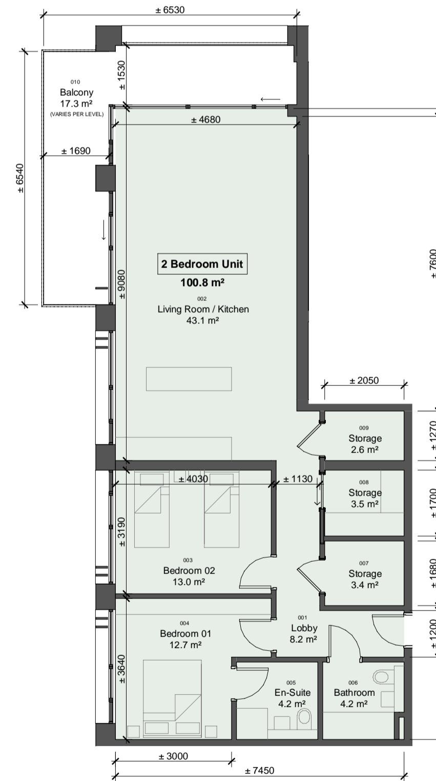
6 Unit Type 2BR-L-1 scale 1 : 100
