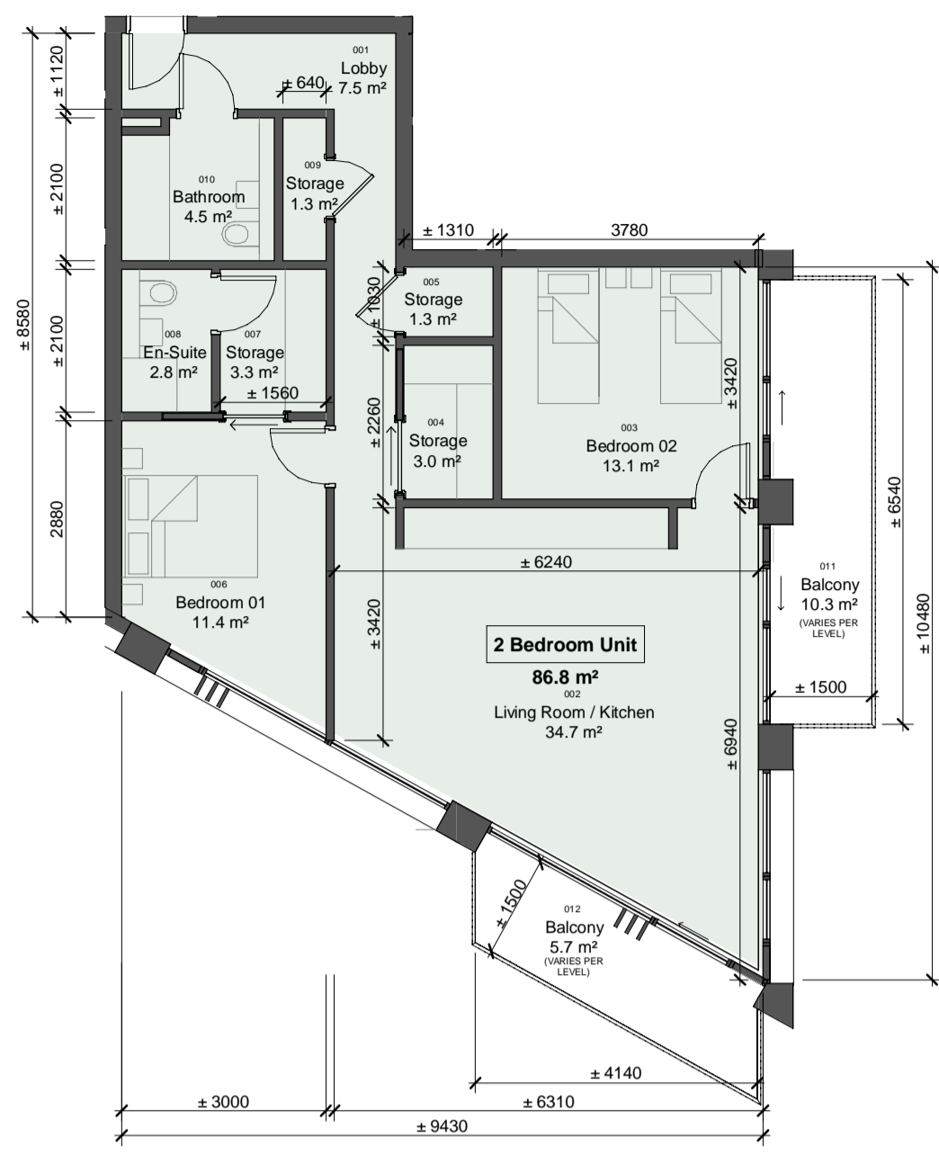
1 Unit Type 2BR-I-1 scale 1 : 100
